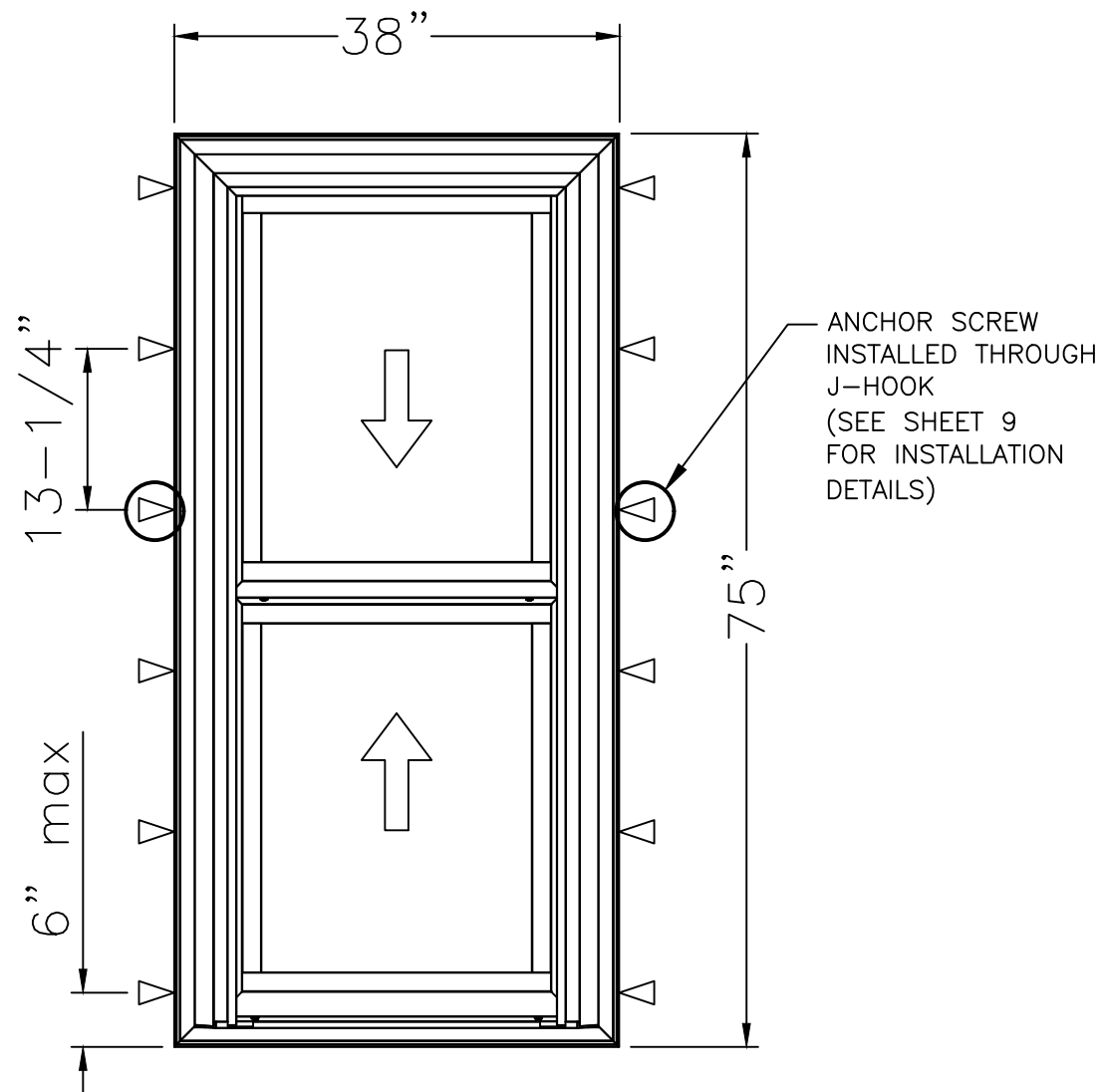
1650i PVC DH WINDOW – FINLESS INSTALLATION MAXIMUM SIZE 38" X 75" DESIGN PRESSURE +60/-70 PSF MISSILE D – WIND ZONE 3
