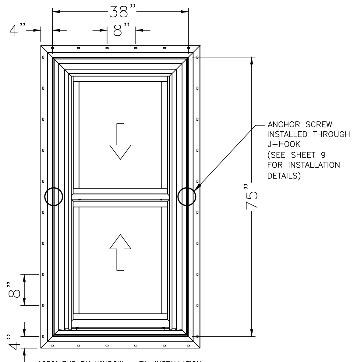
1650i PVC DH WINDOW – FIN INSTALLATION MAXIMUM SIZE 38" X 75" DESIGN PRESSURE +60/-70 PSF MISSILE D – WIND ZONE 3
